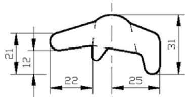
Nova Grip M16 RF
